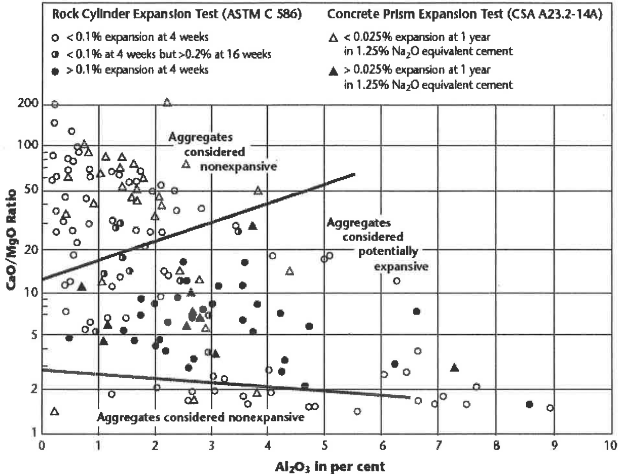
Figure 3. Using Chemical Composition as a Basis for Determining Potential Alkali-Carbonate Reactivity of Quarried Carbonates (from CSA A23.2-26A)
