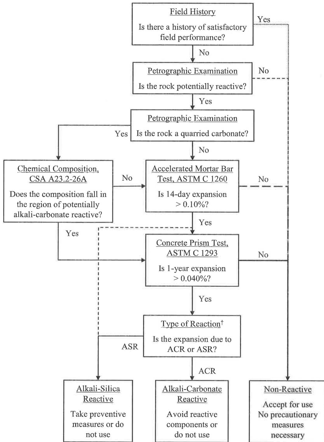
Figure 2. Sequence of Laboratory Tests for Evaluating Aggregate Reactivity
