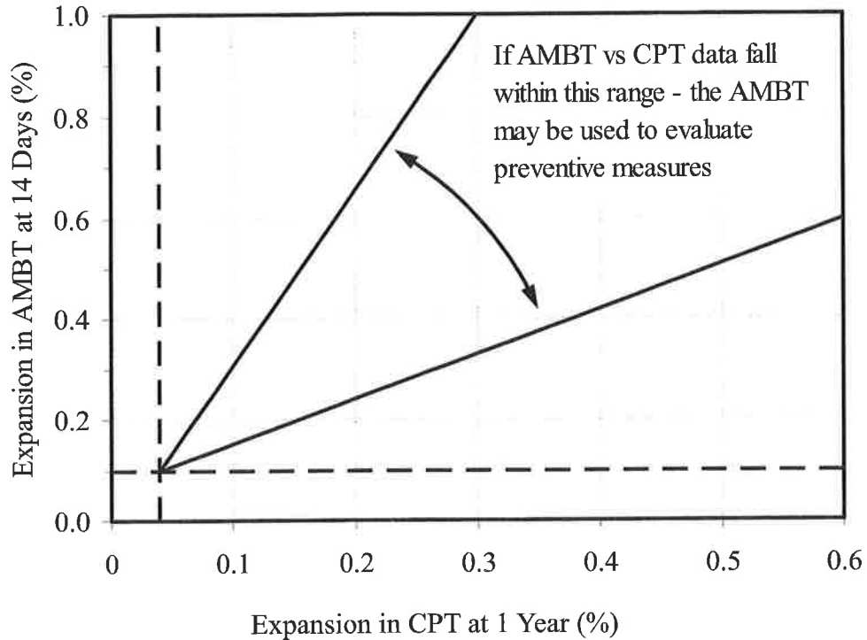
Figure 4. Comparison of AMBT and CPT Data for the Purpose of Determining Whether the AMBT is Suitable for Evaluating Preventive Measures with a Specific Aggregate
