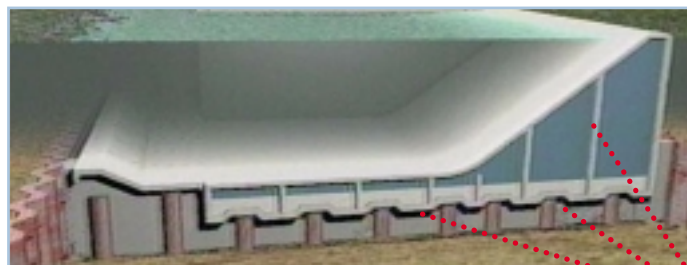
Cast-in-place SLC interior supports and floor sections
